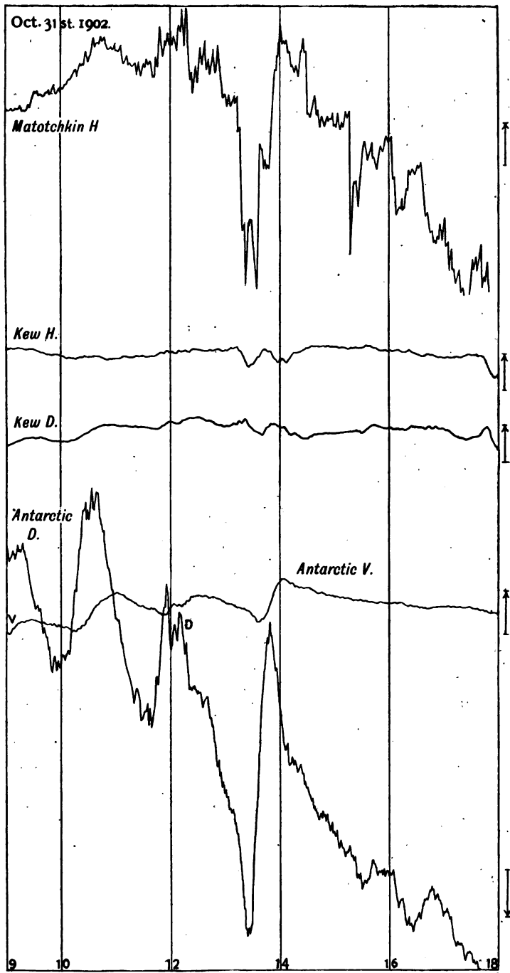
FIG. 30.—ARCTIC-KEW-ANTARCTIC CURVES.
